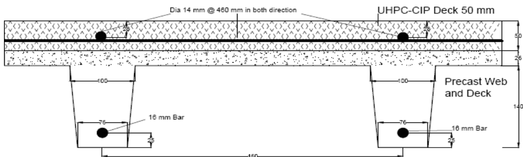
(b) Typical Panel Strip.
