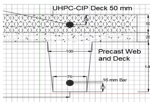
(a) Details of a Typical Rib.
